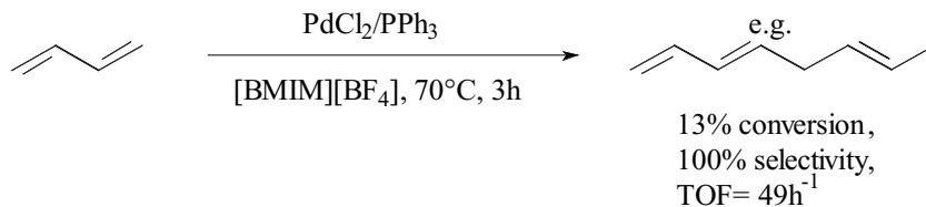
Scheme 5.2-23: Biphasic, Pd-catalyzed dimerization of butadiene in [\text{BMIM}][\text{BF}_4] .
