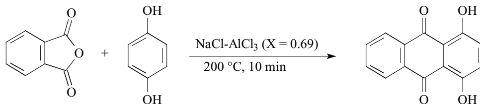
Scheme 5.1-58: The reaction between phthalic anhydride and hydroquinone in NaCl/AlCl 3 ( X(\text{AlCl}_3) = 0.69 ).
