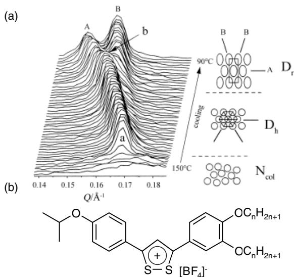
Figure 4.1-8: (a) Small-angle X-ray diffraction data relating to the ditholium salt shown in (b) for n = 12 . A and B correspond to the rectangular lattice vectors shown in \text{D}_{\text{r}} , and a and b correspond to the \text{N}_{\text{col}} to \text{D}_{\text{h}} and \text{D}_{\text{h}} to \text{D}_{\text{r}} phase transitions. Reproduced from reference 30 with permission.
