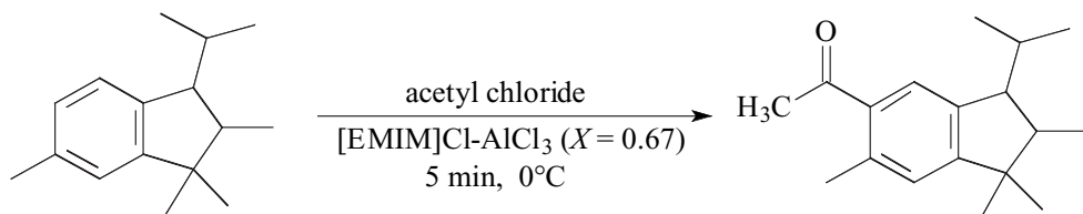
Scheme 5.1-63: The acetylation of 1,1,2,6-tetramethyl-3-isopropylindane in [EMIM]Cl/AlCl 3 ( X(\text{AlCl}_3) = 0.67 ).
