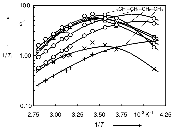
Figure 4.5-1: ^{13}\text{C} relaxation rates 1/T_1 of [BMIM][PF 6 ] in the neat liquid as a function of reciprocal temperature T ( \Delta : C2, \square and \diamond : C4 and C5, X: CH 3 (ring), +: CH 3 (butyl group), \circ : CH 2 , lines: functions calculated with the fitted parameters).
