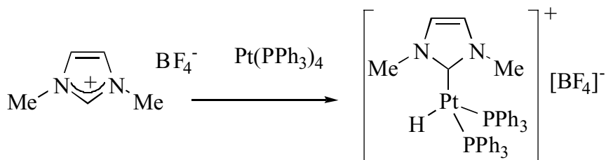
Scheme 5.3-3: Formation of carbene complexes by oxidative addition to \text{Pt}(0) .
