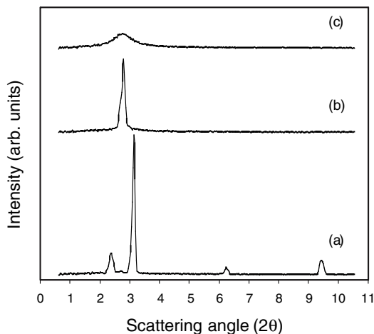
Figure 4.1-7: Small-angle X-ray diffraction data from [\text{C}_{16}\text{MIM}][\text{OTf}] at (a) 50 °C, (b) 70 °C, and (c) 90 °C, in the crystal, \text{SmA}_2 , and isotropic phases, respectively, on cooling. Reproduced from reference 27 with permission.
