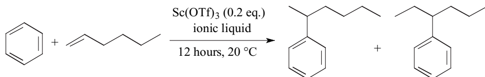
Scheme 5.1-55: The alkylation of benzene with hex-1-ene, catalyzed by scandium(III) triflate in ionic liquids.
