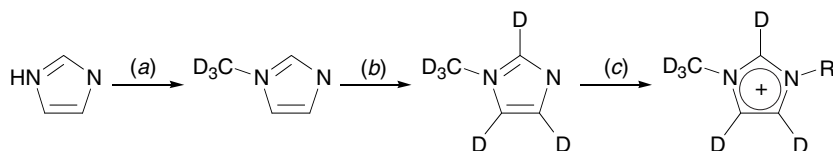
Scheme 4.1-1: Reaction scheme showing a method for deuteration of 1-alkyl-3-methylimidazolium salts: (a) \text{CD}_3\text{OD} , \text{RuCl}_3/(\textit{n}\text{-BuO})_3\text{P} , (b) \text{D}_2\text{O} , 10 % Pd/C, and (c) RX ( \text{CD}_3\text{Cl} , \text{C}_2\text{D}_5\text{I} ).
