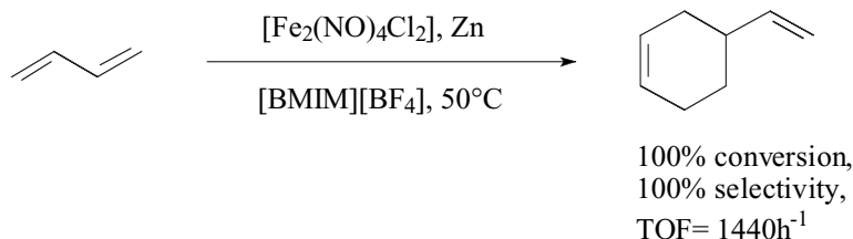
Scheme 5.2-24: Biphasic, Fe-catalyzed cyclotrimerization of butadiene in [\text{BMIM}][\text{BF}_4] .
