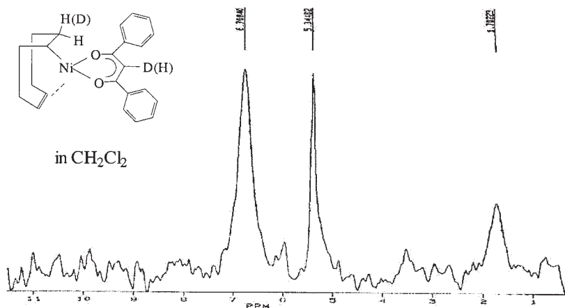
Figure 5.2-3: ^2\text{H} NMR spectra of the deuterated analogue of the square planar Ni-complex ( \eta -4-cycloocten-1-yl)(1,5-diphenyl-2,4-pentanedionato-O,O')nickel recorded [EMIM]Cl/AlCl 3 [X(AlCl 3 ) = 0.55] and in CH 2 Cl 2 .
