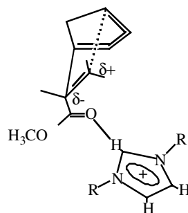
Figure 3.5-3: The hydrogen bond (Lewis acid) interaction of an imidazolium cation with the carbonyl oxygen of methyl acrylate in the activated complex of the Diels-Alder reaction.
